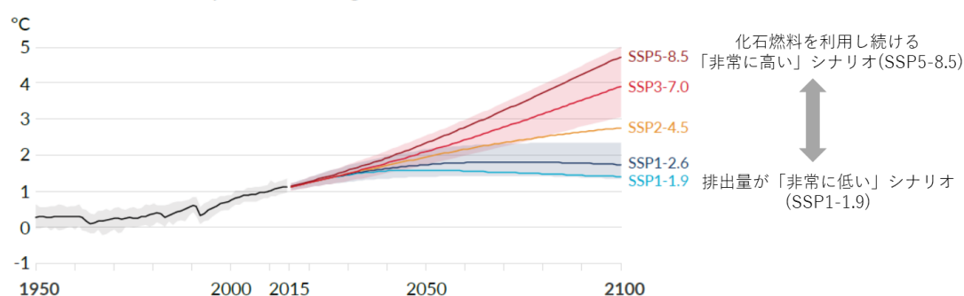
a) Global surface temperature change relative to 1850-1900
